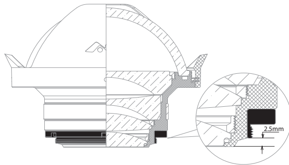
TYPE B Adaptor (3B043300-4LC01)
