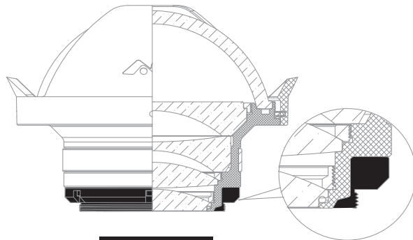
TYPE A Adaptor Pre-assembled (3B043400-4LC01)
